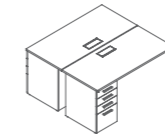
DE69-5.12k W1200•D1212•H750 DE69-5.14k W1400•D1412•H750 DE69-5.15k W1500•D1412•H750 DE69-5.16k W1600•D1412•H750
