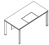
DE88-5.16 W1600•D800•H750 DE88-5.18 W1800•D900•H750 DE88-5.20 W2000•D1000•H750
