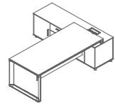
DE87(L/R)-5.21 W2100•D1900•H750 DE87(L/R)-5.23 W2300•D1900•H750
