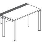
DE67-5.12F W1200•D730•H750 DE67-5.14F W1400•D730•H750 DE67-5.15F W1500•D830•H750 DE67-5.16F W1600•D830•H750
