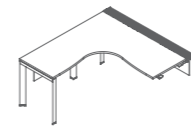
DE630(L/R)-5.14F W1400•D1530•H750 DE630(L/R)-5.15F W1500•D1630•H750 DE630(L/R)-5.16F W1600•D1730•H750
