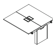
DS625 Middle Workstation Of Double Row W1200•D1212•H750 W1400•D1412•H750 W1500•D1412•H750 W1600•D1412•H750
