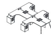
DS56.14/15/16 W2800•D2710•H750 W3000•D2710•H750 W3200•D2710•H750
