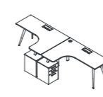
DS51.14/15/16 W2800•D1355•H750 W3000•D1355•H750 W3200•D1355•H750
